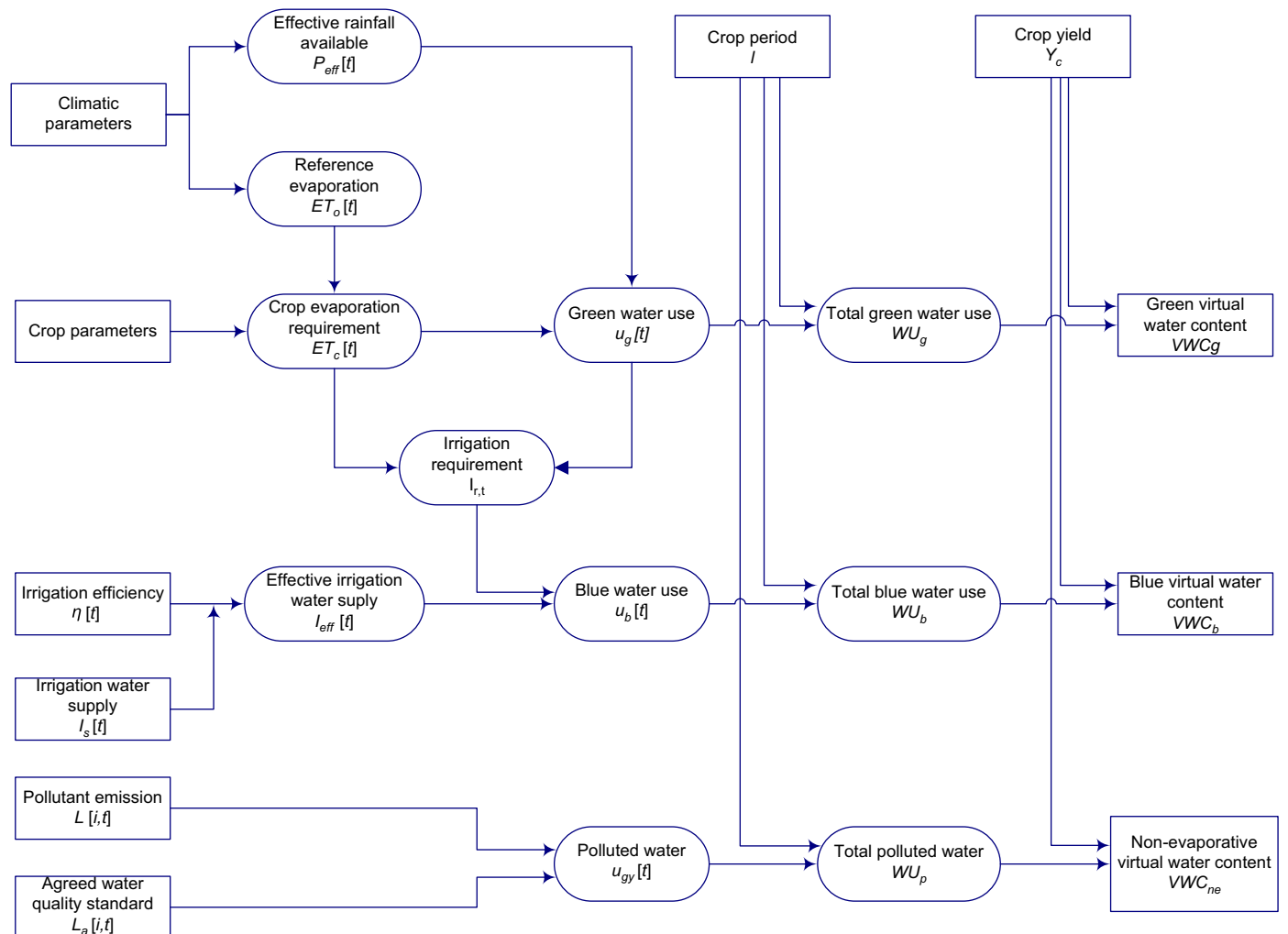
Fig. 1. Diagram to calculate the virtual water content of a primary crop grown without cover.
